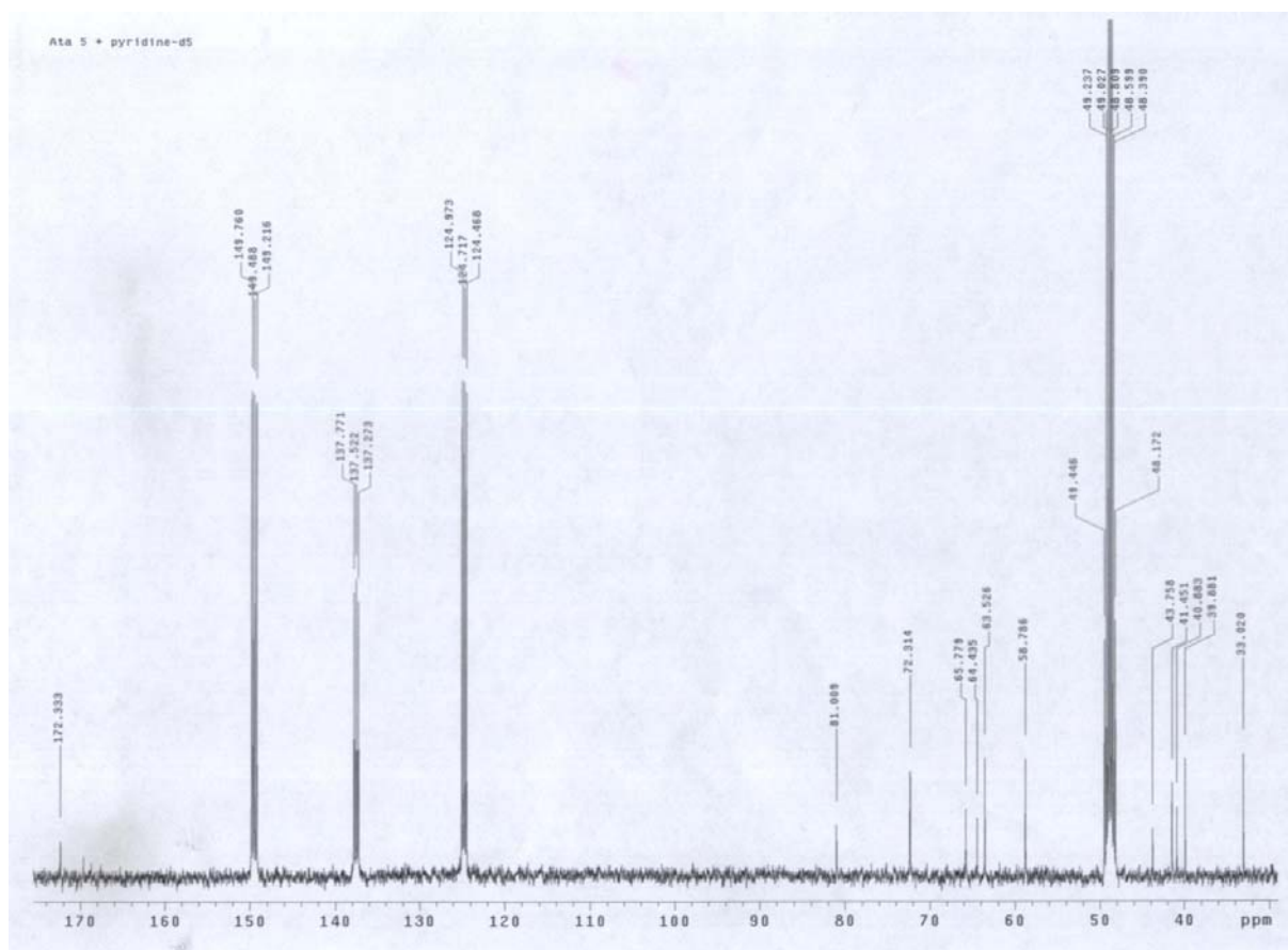
13 C-NMR Spectrum
