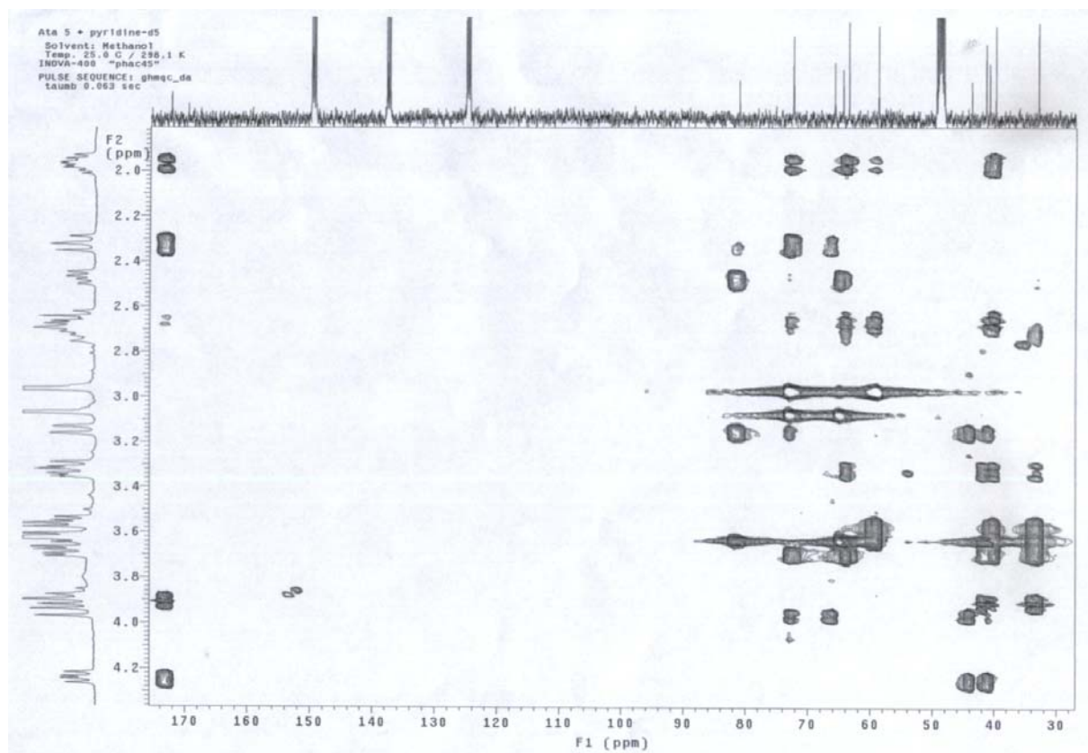
HSQC Spectrum
