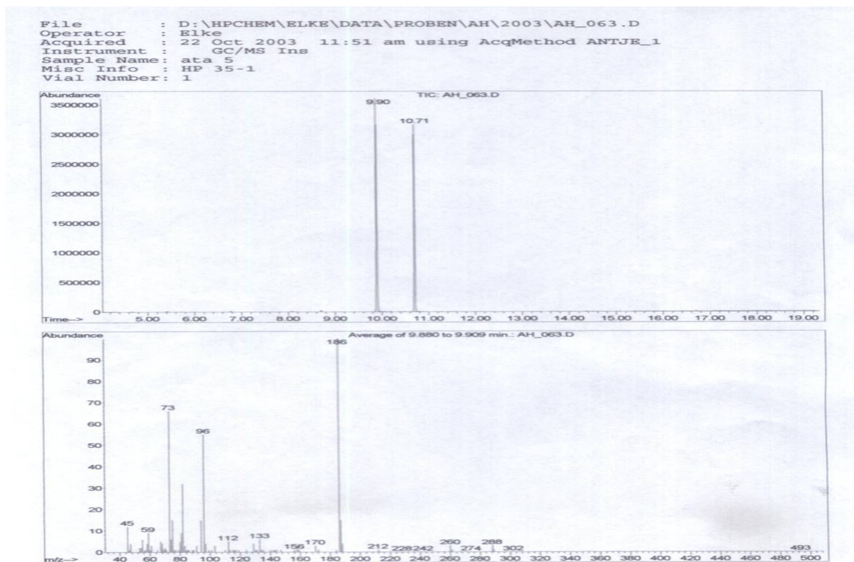
GC-MS of compound 1B
