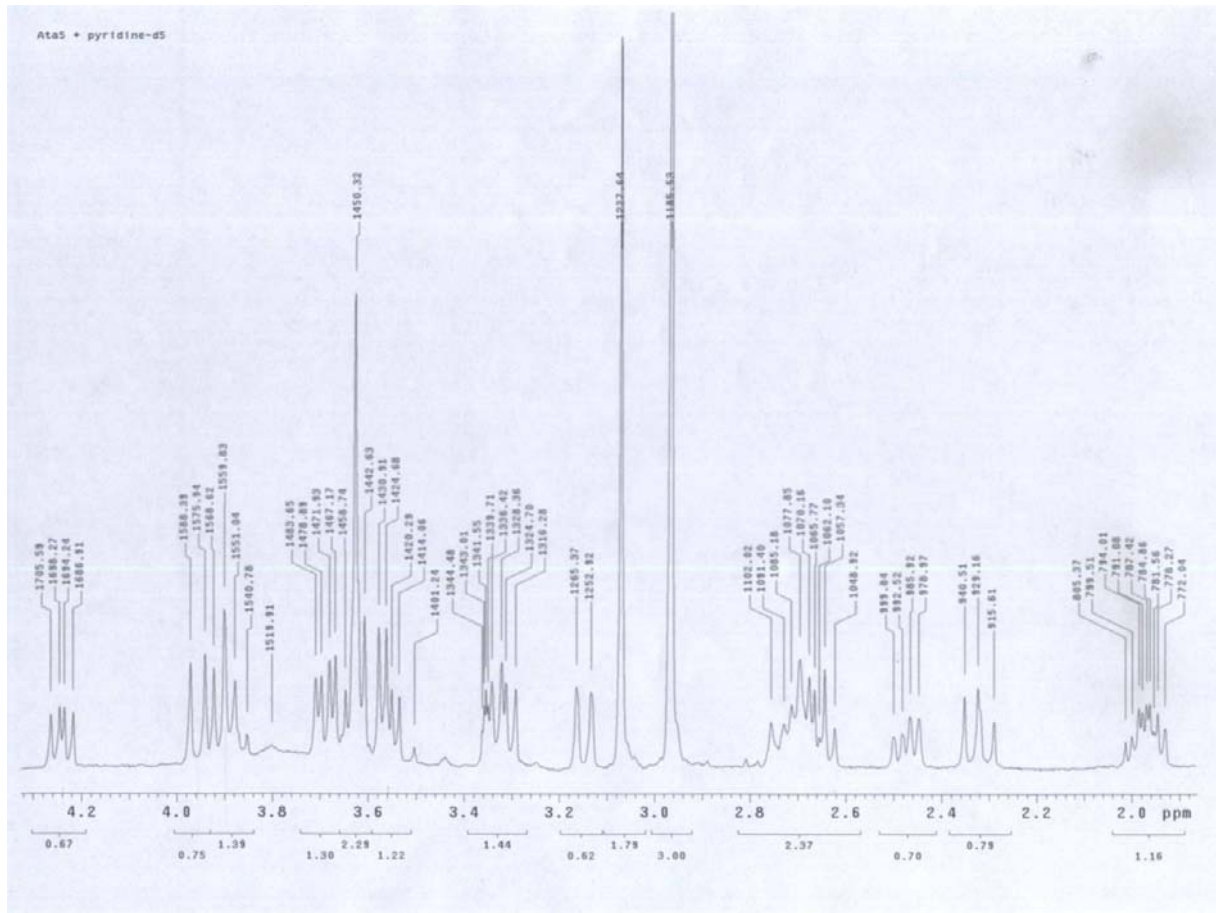
1 H-NMR Spectrum
