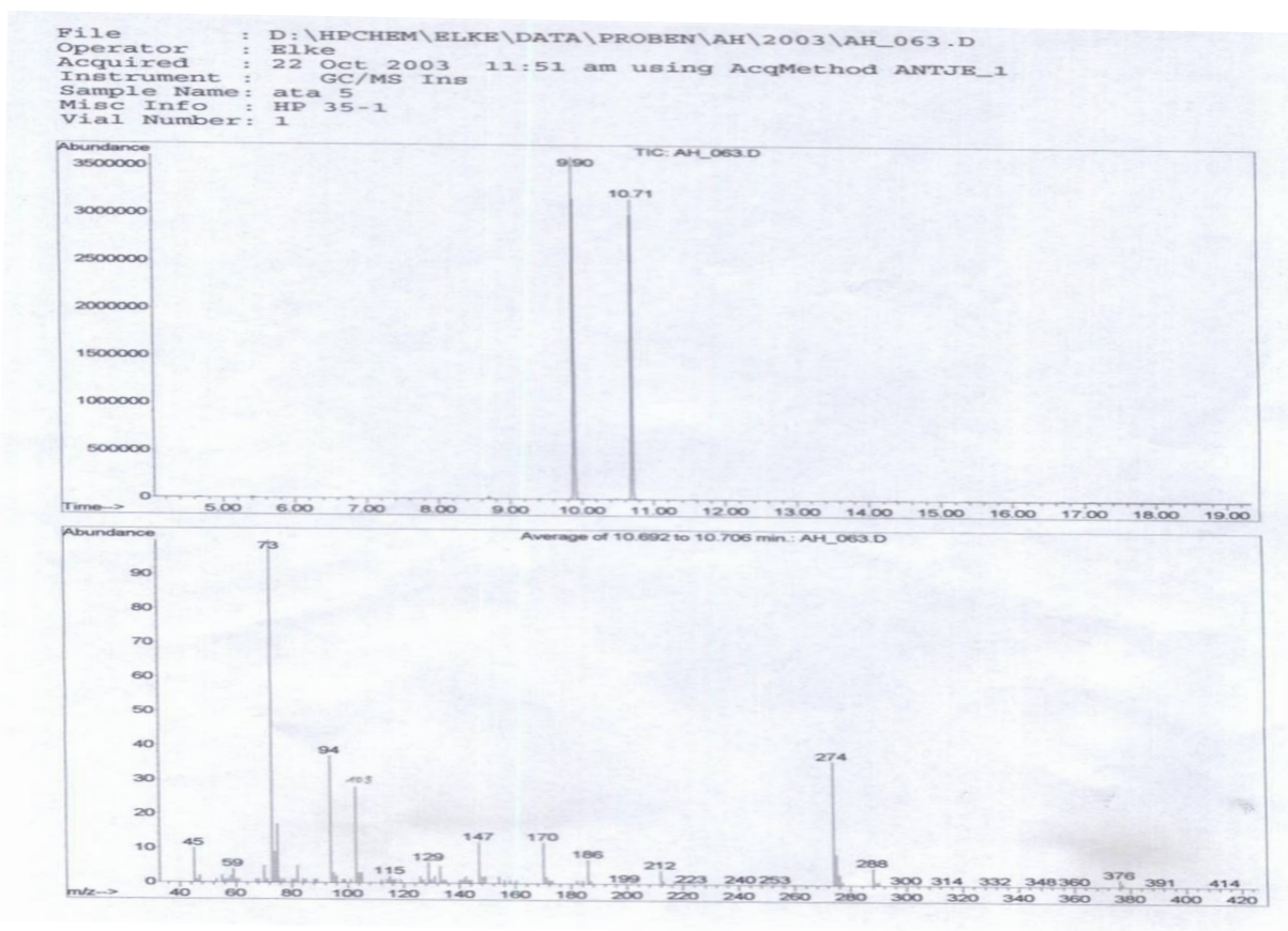
GC-MS of compound 1A
